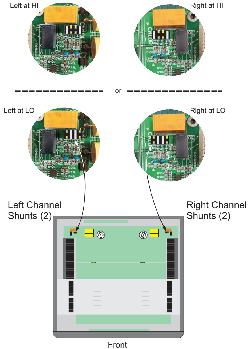
Figure 9 – Internal Gain Jumper Settings
