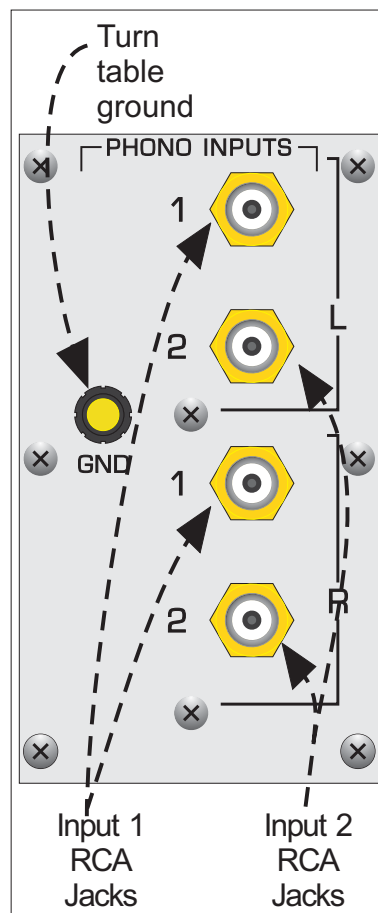
Figure 6 – Phono Module
