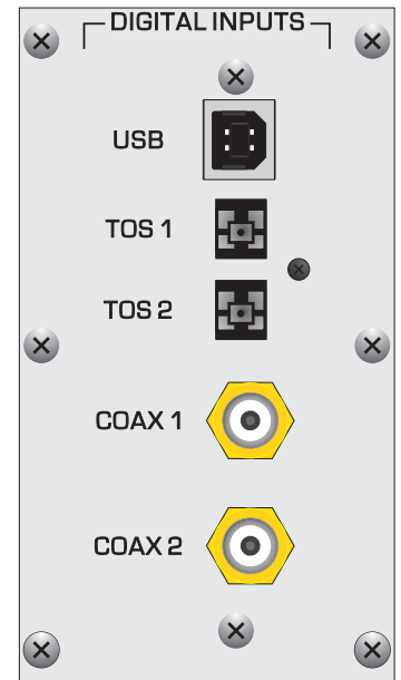
Figure 8 – DAC Module
