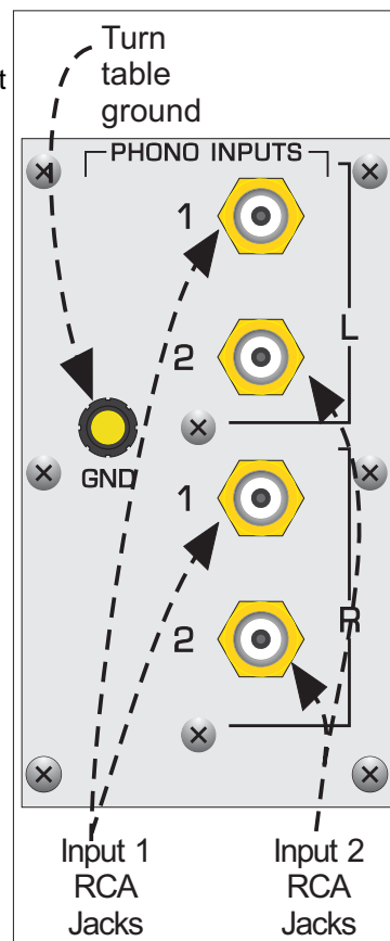
Figure 6 – Phono Module
