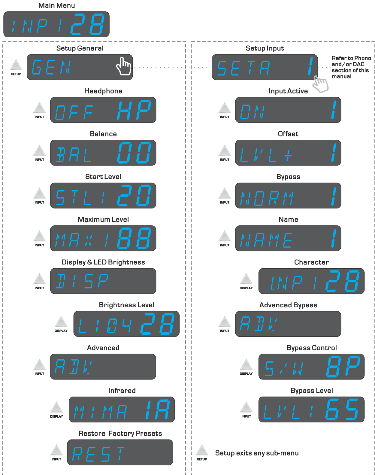
Figure 4 – Mimas Standard Menus
